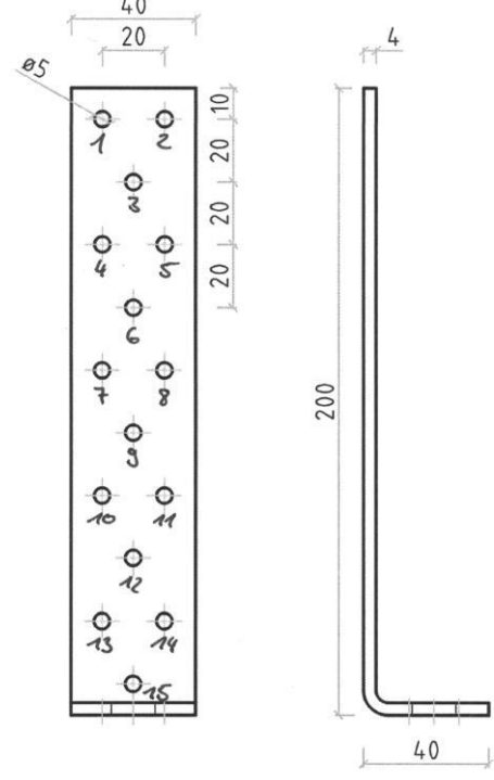
Figure B. 1 Dimensions of type WZU 15550
