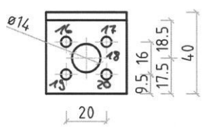
Figure B. 3 Dimensions of type WZU2004
